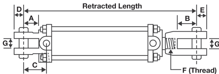
Dimensional Data for Prince Tie Rod Cylinders
